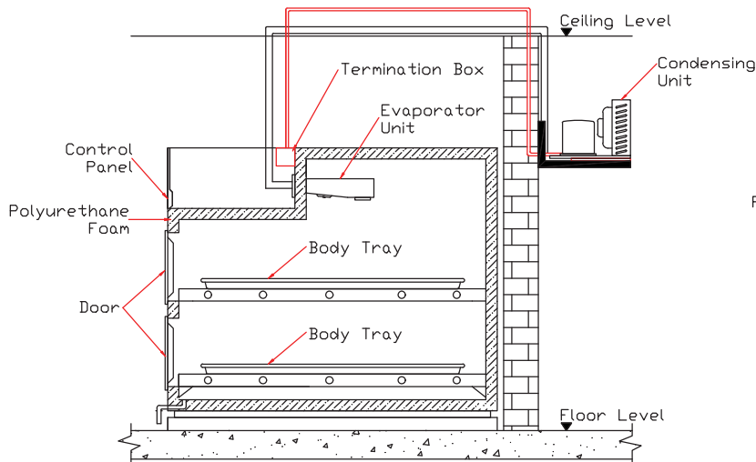
Side View Model : 2201-RA (Remote Type Compressor)
