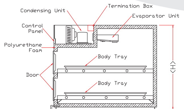
Side View Model : 2201-FA (Front Compressor)
