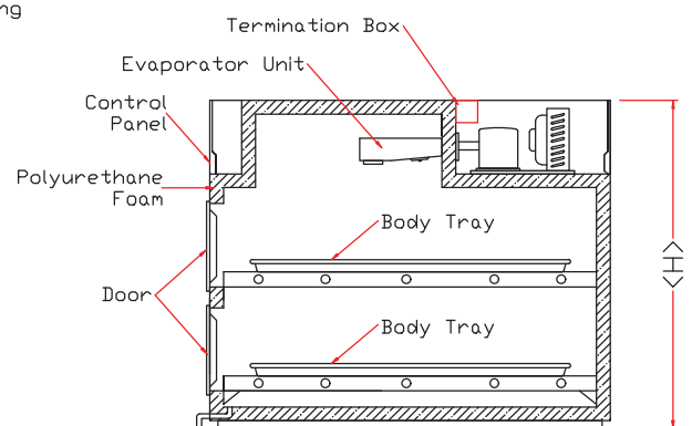
Side View Model : 2201-BA (Back Compressor)
